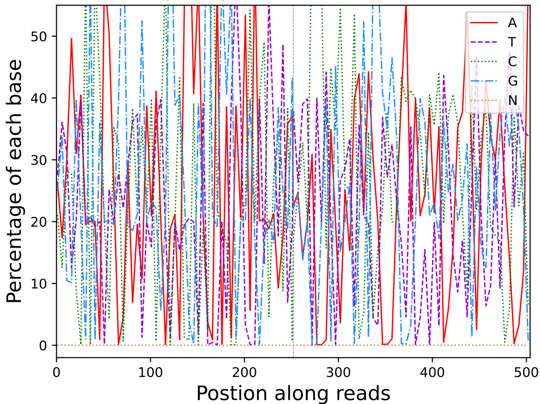
Base percentage along reads (R10216)
